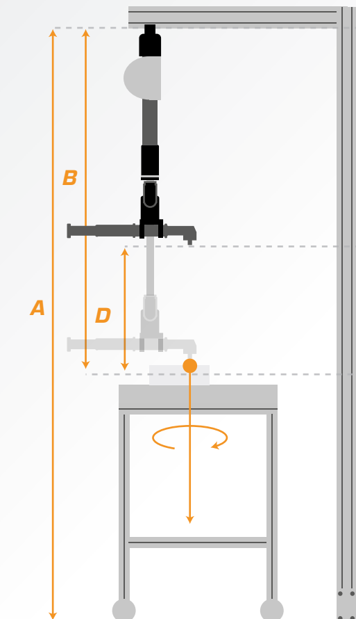
Ex. 7: Floor mounted BRV with angle screwdriver
