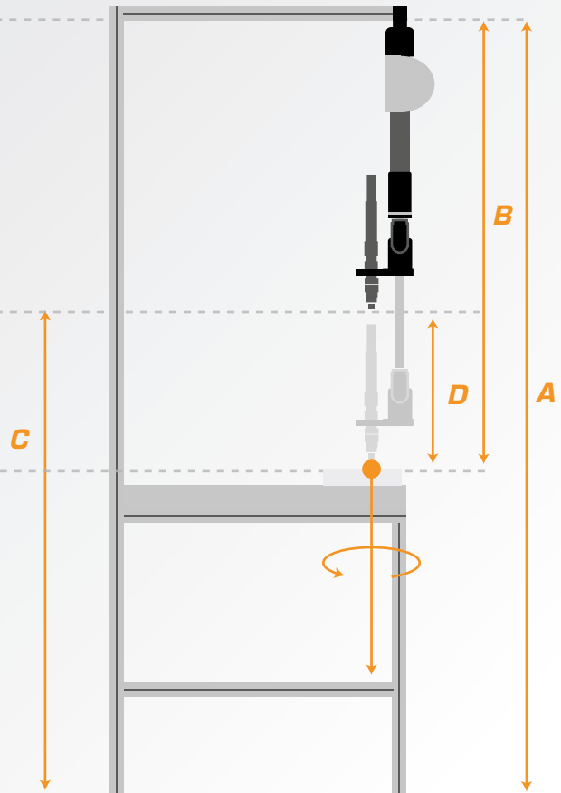
Ex. 6: BRV mounted on workstation with straight screwdriver
