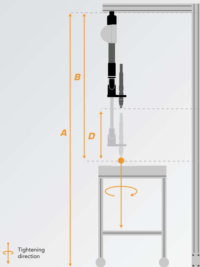
Ex. 5: Floor mounted BRV with straight screwdriver
